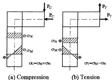
Fig. 2 Calculation of Yield Strength ( P_y )
