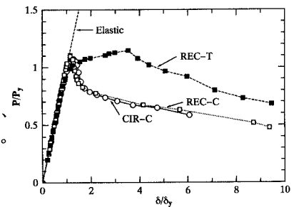
Fig. 3 Relation between Load and Displacement for Static Loading
