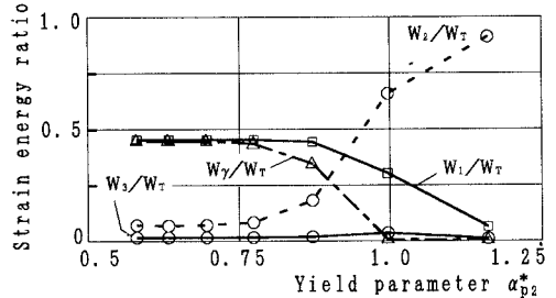
(b) Absorbed strain energy ratio Fig. 4 Variation of cumulative strain and absorbed energy every cross-section due to yield parameter
