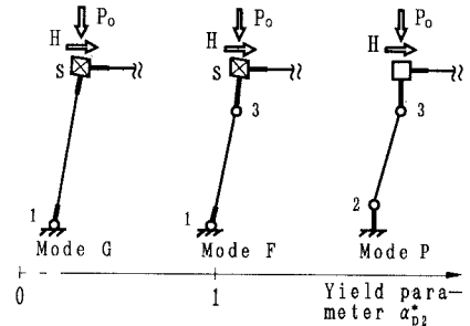
Fig. 2 Fundamental collapse patterns (□, ○: Plastic deformation)
