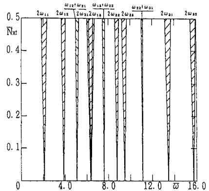
図-2 動的不安定領域 (CASE I, \beta = 1.0, \theta = 30^\circ )
