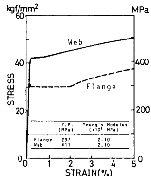
Fig.3 Tensile stress-strain relations
