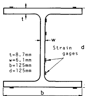
Fig.2 Measurement of curvature
