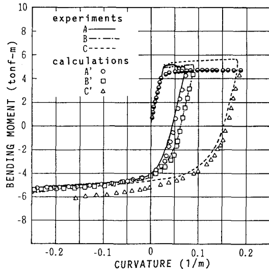
Fig.6 Measured and calculated moment-curvature relations
