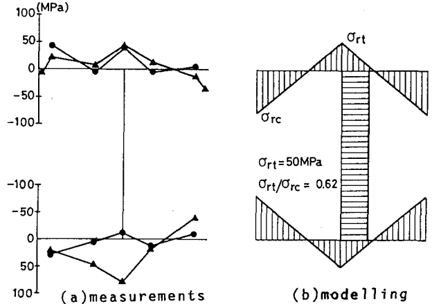
Fig.5 Residual stress distribution
