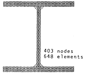
Fig.4 Mesh pattern
