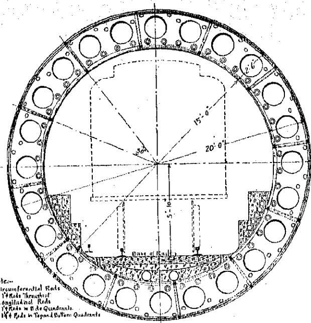
Assembled Ring—Recess Side
