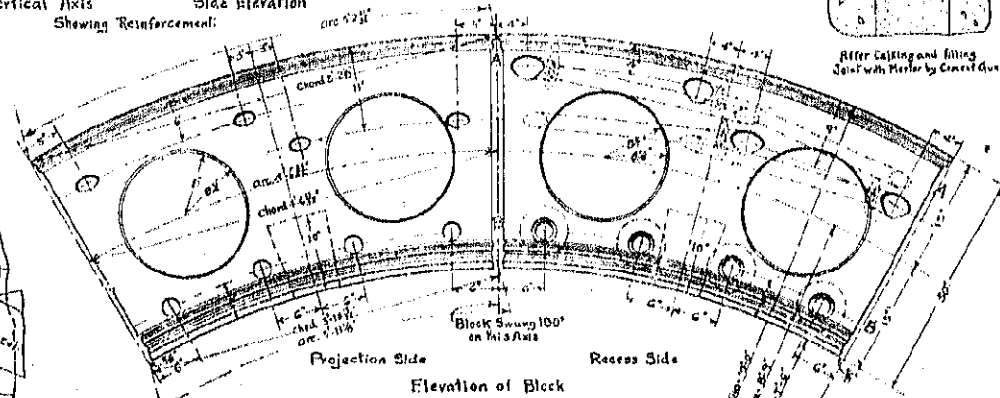
Elevation of Block
