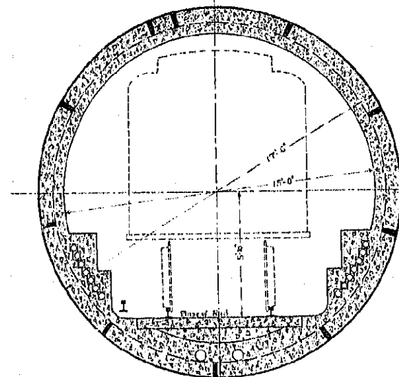
Present Cast Iron Section
