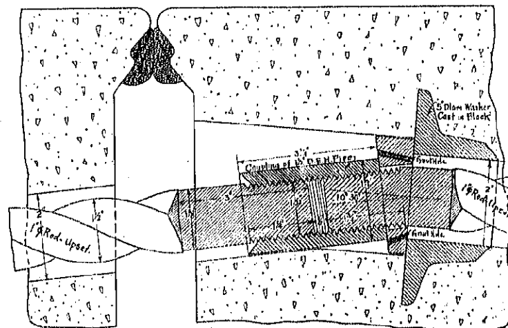
Detail of Joint for Diagonal Rods. Section along E of Rods
