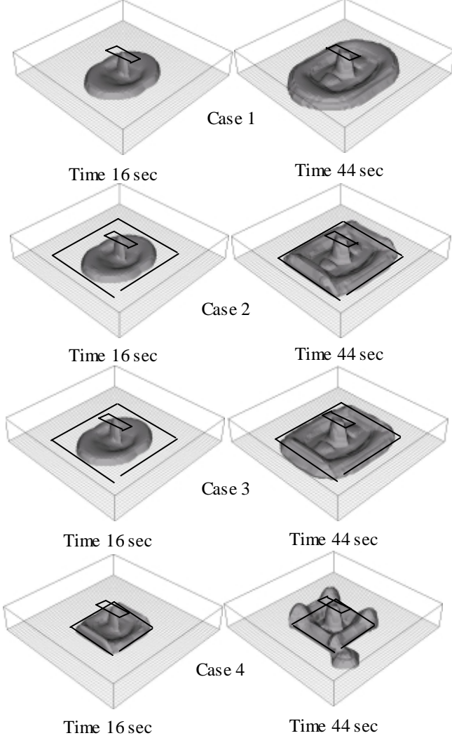
Fig. 12 Simulated currents under the different positions and height of the fence.
