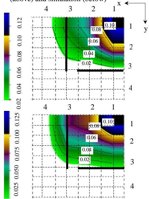
Fig.10 Contours of W_d^* for case 2. Experiment (above) and simulated (below)
