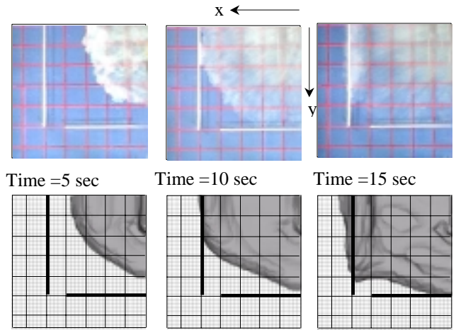
Fig.9 Spreading of the current for case 2. Experiment (above) and simulation (below)
