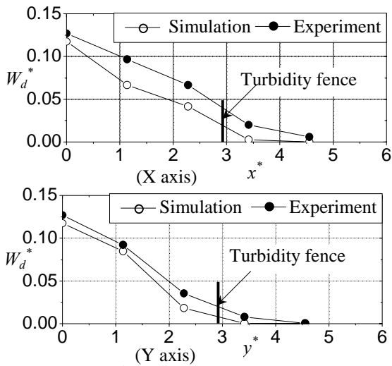
Fig. 8 W_d^* along the X axis (above) and the Y axis (below) for Case 1.
