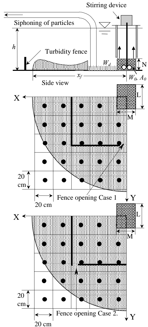
Fig.1 Schematic diagram showing the 3D gravity current and experimental set up.
