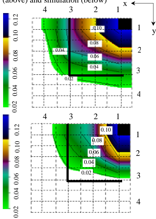
Fig. 7 Contours of W_d^* for case 1. Experiment (above) and simulated (below)
