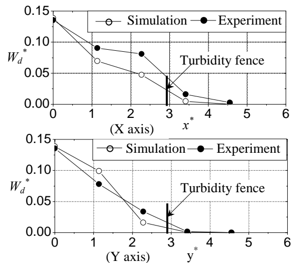
Fig.11 W_d^* along the X axis (above) and the Y axis (below) for Case 2.
