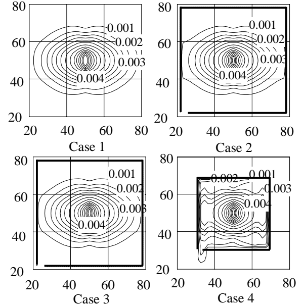
Fig. 13 Simulated contours of W_d^* under the different positions and height of fence.
