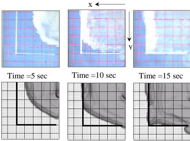
Fig.6 Spreading of the current for case 1. Experiment (above) and simulation (below)
