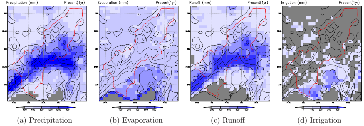
Fig. 4 Annual water balance components of the present run
