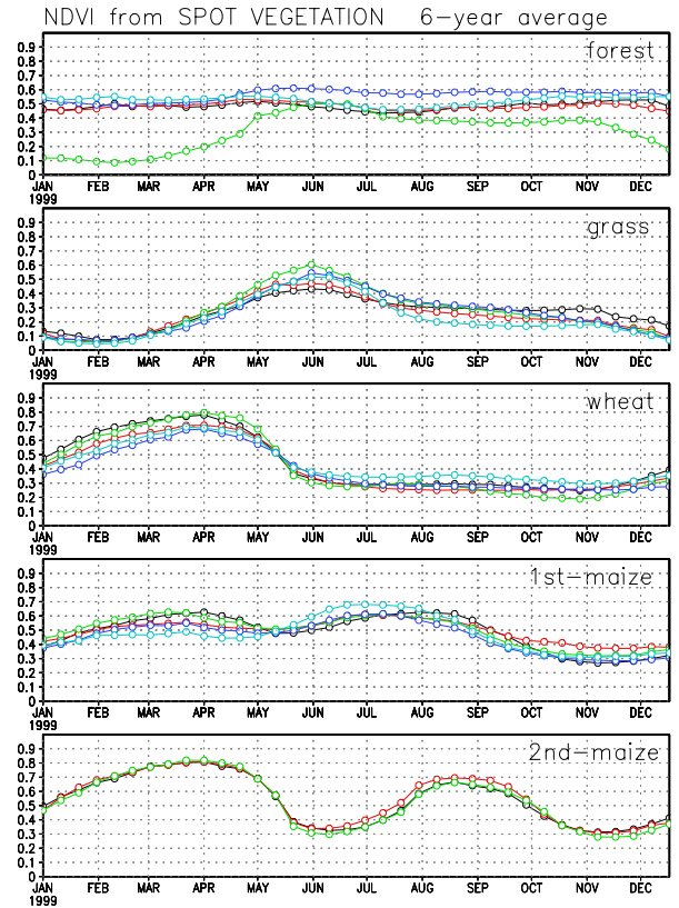
Fig. 1 Average annual time series of NDVI at different landcover conditions. Several lines in one panel correspond to each GCP in Table1.
