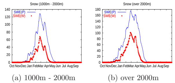
Fig. 6 Snow water equivalent (daily)
