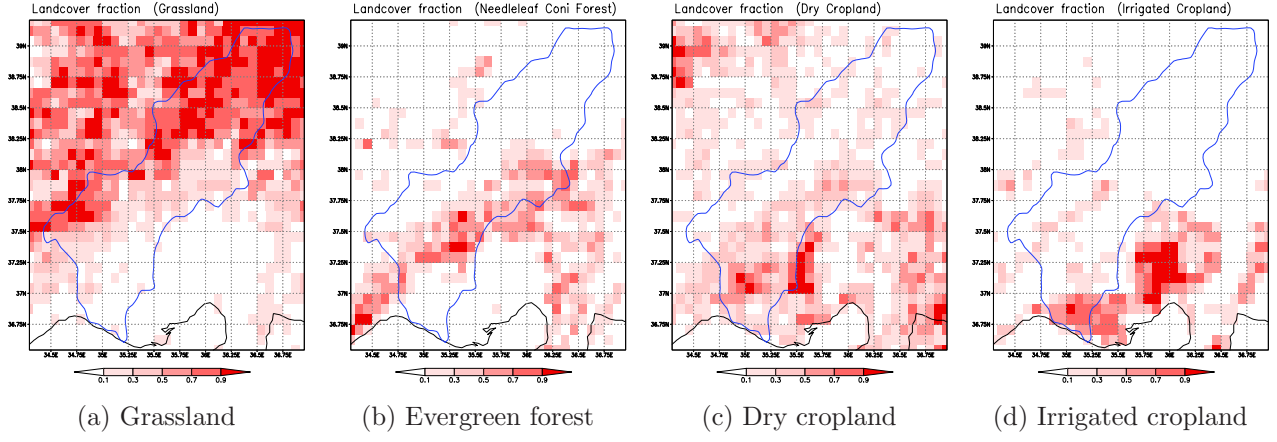
Fig. 3 Landcover fraction of each grid (5 min resolution)
