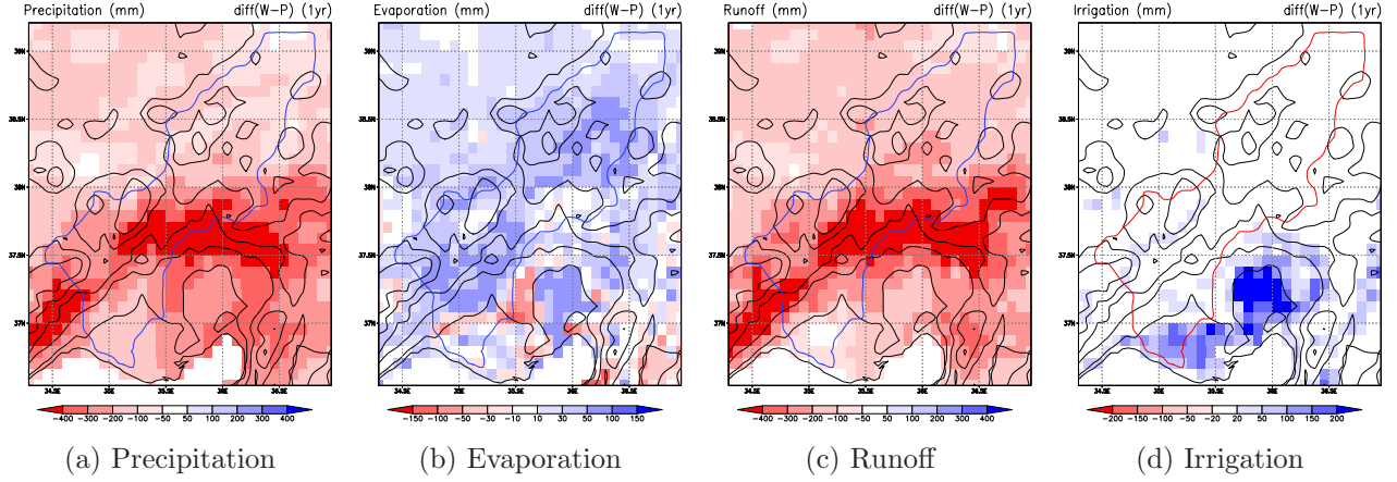
Fig. 5 Difference (Future - Present) of annual water balance components
