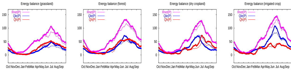
(a) Surface energy balance components (15days running mean) Rnet: net radiation, Qle: latent heat, Qh: sensible heat
