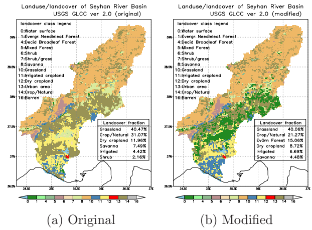
Fig. 2 Original and modified landcover information of the Seyhan River Basin
