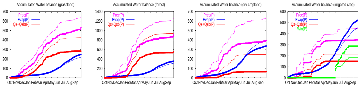
(b) Accumulated water balance components (daily) Prec: precipitation, Evap: evaporation, Qs+Qsb: runoff, Win: irrigation
