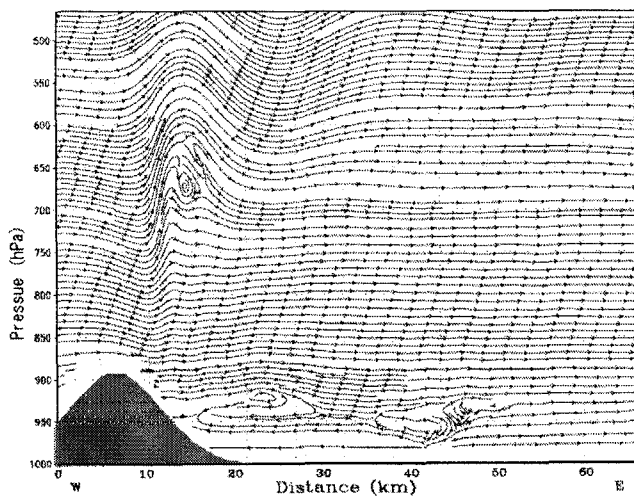
Fig. 6 Streamlines for the 25m/s, 1200m ridge height case. In addition to the rotor beyond the lee slope, there is a vortex above the lee-side slope also. Fr_u=2.1 , Fr_l=0.8
