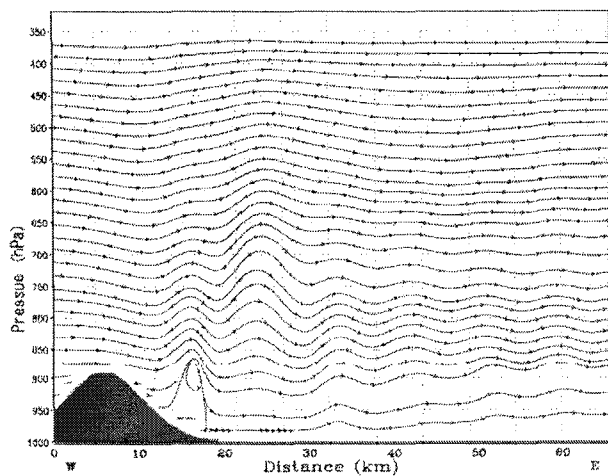
Fig. 5 Lee wave train generated for 35m/s case with 1000m ridge (Streamlines). Fr_u=3.5 , Fr_l=1.2 .
