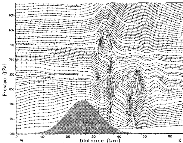
Fig. 10 Streamlines at 1h after transition of background flow from 10m/s to 5m/s. Fr_u=1.3 , Fr_l=0.6
