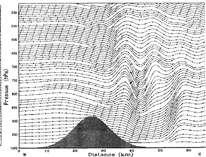
Fig. 9 Streamlines for the case with 10m/s, just before start of the decreasing the wind to 5m/s. Fr_u=2.1 , Fr_l=1.3 .
