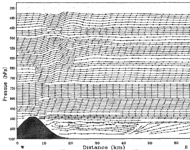
Fig. 4 Case with U=10\text{m/s} , 1000m ridge. Note the propagation of lee waves almost vertically upwards. In this case the waves are not trapped. Fr_u=1 , Fr_l=0.4
