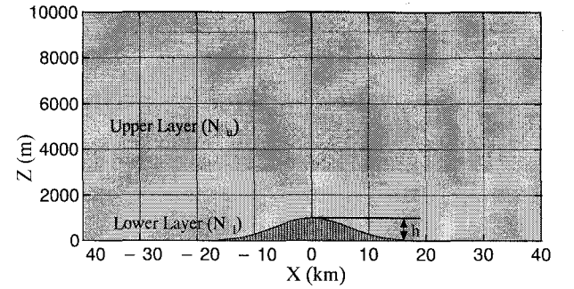
Fig. 2 Model setup. N_u and N_l indicate the Brunt-väisälä frequency of the upper and lower layers. Mountain profile is defined by z = h \exp(-x^2/b^2) , where h is the maximum height.
