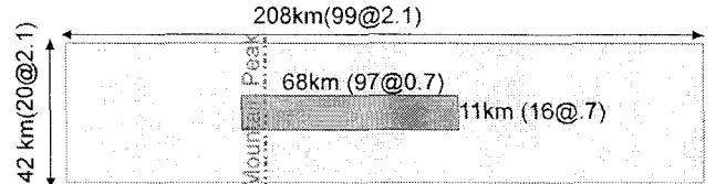
Fig. 3 Numerical setup. A high-resolution (0.7km) grid of 97x16 was nested inside the coarser (2.1km) grid of 99x20. Vertical space was divided into 50 grids with unequal spacing.
