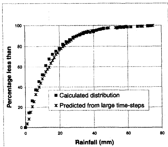
Fig. 13 Comparison of cumulative event volume distribution at 10min resolution.
