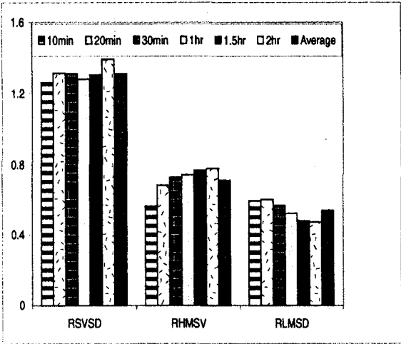
Fig. 9 Values of power-factors at various resolutions.
