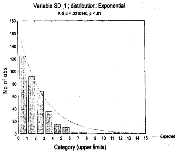
Fig. 6 Probability distribution for SD.
