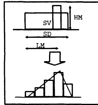
Fig. 2 Constructing a rain storm using the model output.
