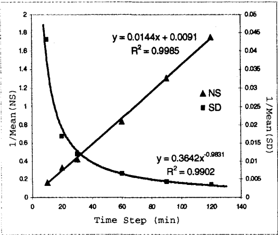
Fig. 10 Scaling of the means of NS and SD.
