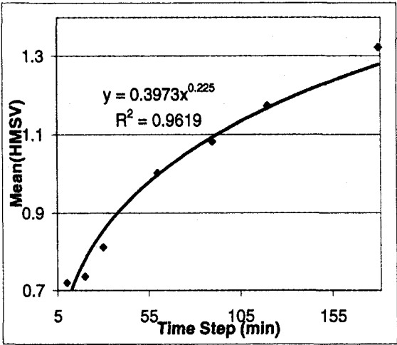
Fig. 12 Scaling of the mean of HMSV.
