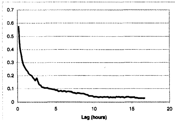
Fig. 4 Autocorrelations of the rainfall data.
