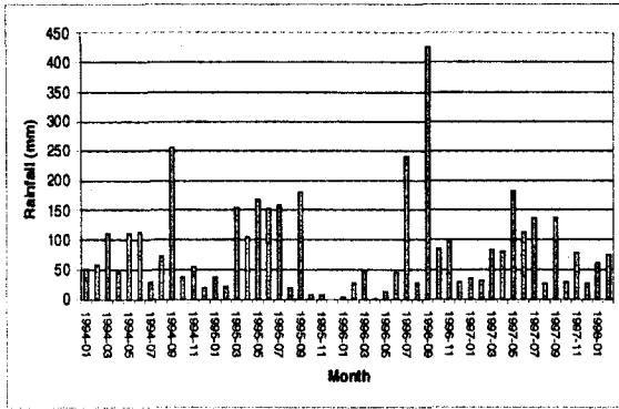
Fig. 3 Monthly average rainfall values of the available rainfall data.
