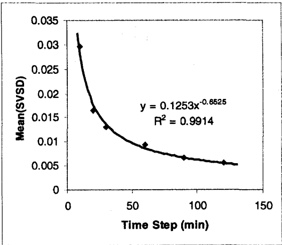
Fig. 11 Scaling of the mean of SVSD.
