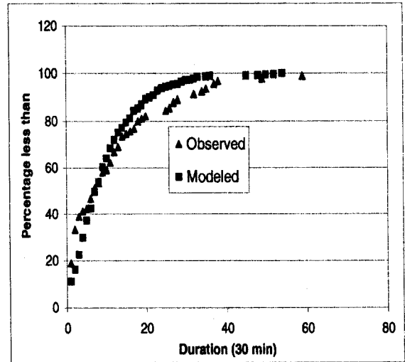
Fig. 7 Event duration distributions at 30min resolution.
