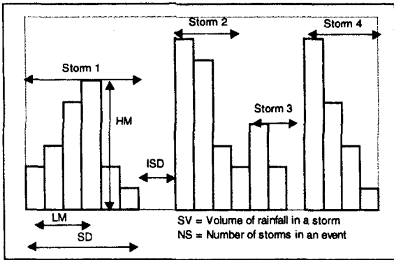
Fig. 1 Six parameters used to describe the structure of a rain event.
