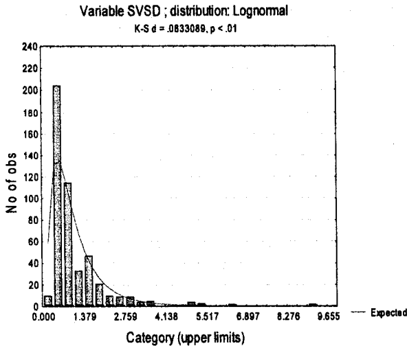
Fig. 5 Probability distribution for SVSD.
