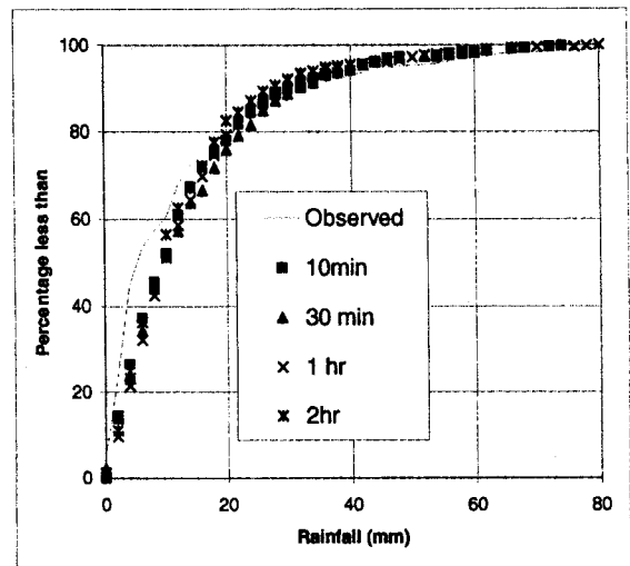
Fig. 8 Event volume distributions.
