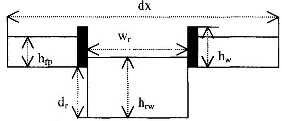
Fig 2: Concept of flow exchange between river and surface grids considering embankment heights
