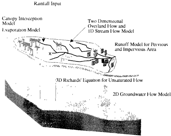
Fig. 1: Schematic diagram of a distributed hydrologic model
