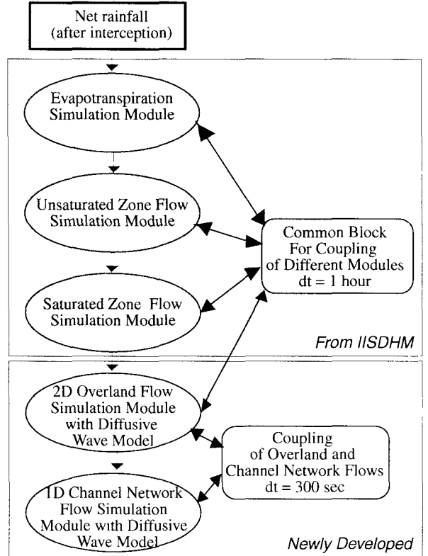
Fig. 3: Flow chart showing coupling process of distributed model
