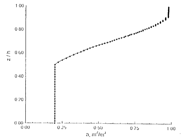
Figure 1: Distribution of leaf area density in the plant canopy
