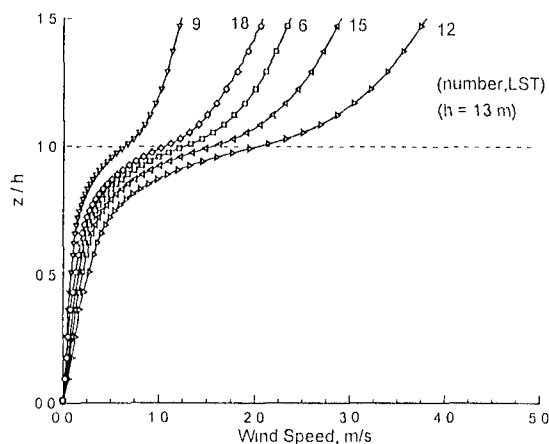
Figure 6: Computed wind velocity profile in the plant canopy (Sept. 1, 1997)
