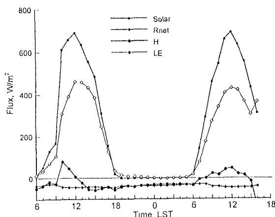
Figure 5: Computed heat balance in the plant canopy (Sept. 1-2, 1997).
