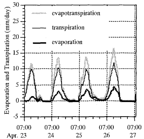
Fig.5 Components in evapotranspiration
