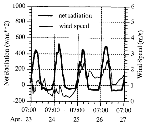
Fig.3 Observations of net radiation and wind speed
