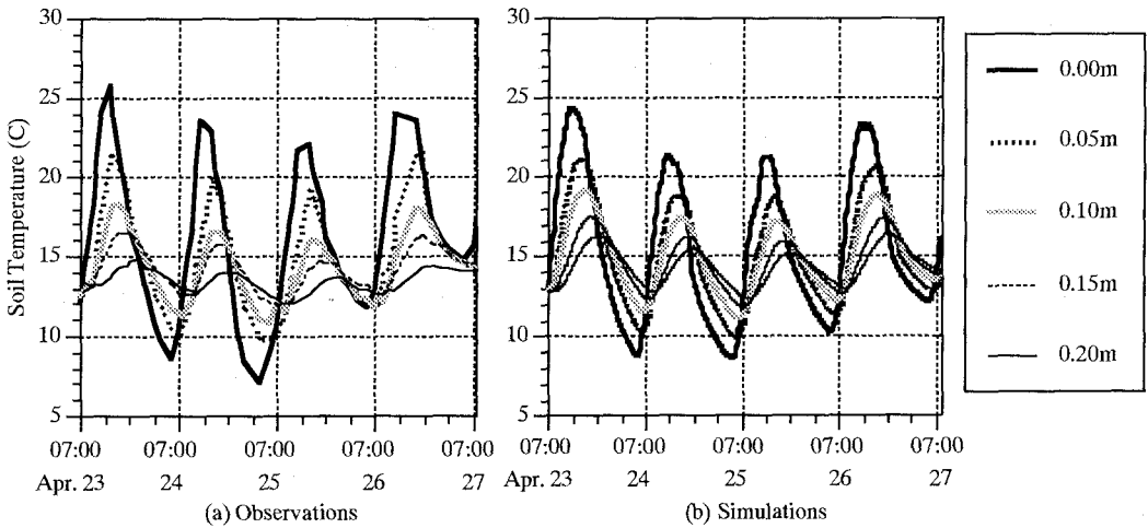
Fig.6 Observations and simulations of soil temperatures in depths of 0.00m, 0.05m, 0.10m, 0.15m, 0.20m
