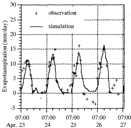
Fig.4 Comparison of evapotranspiration
