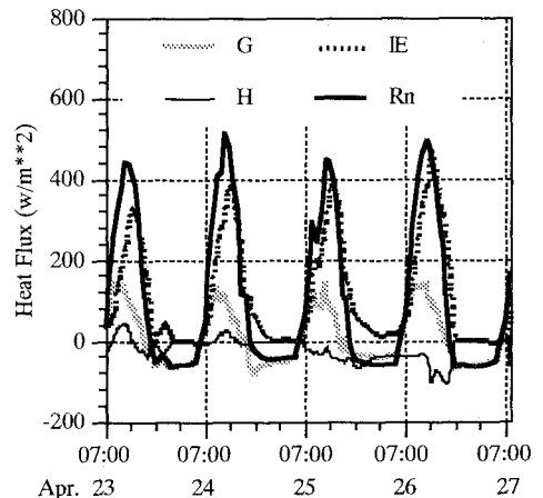
Fig.7 Ground Surface Energy Budget
