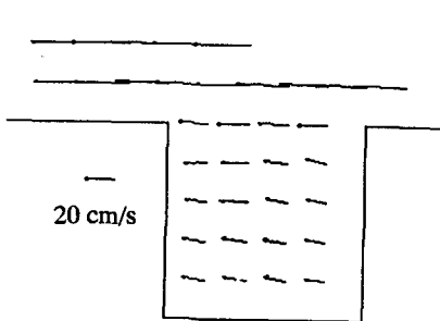
Fig. 12. Velocity field in z_3 plane for flood flow condition.
