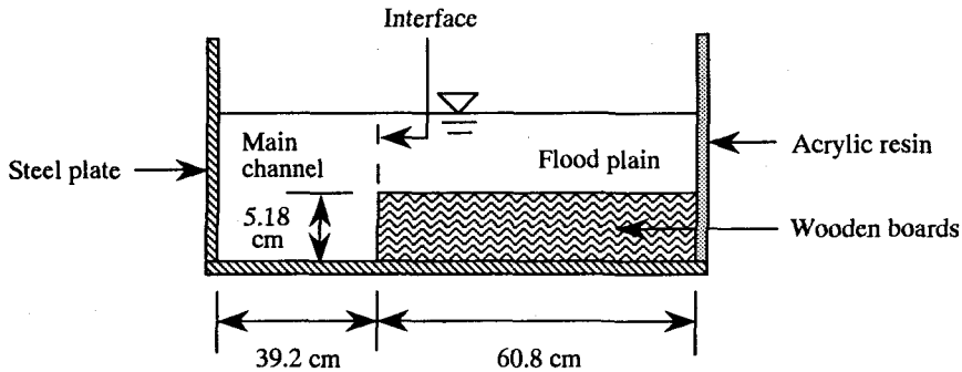
Fig. 2. Cross-section of the compound channel
