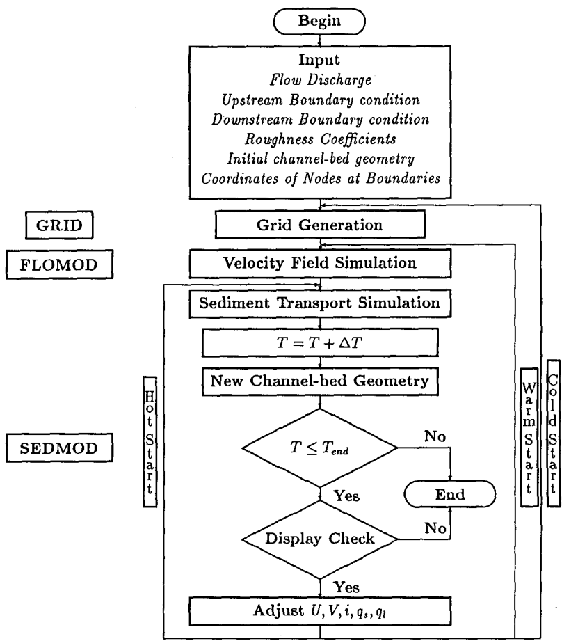
Figure 1: General flowchart
