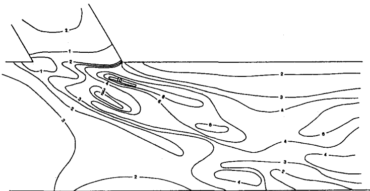
Fig.5 Relative bed shear stress contours
