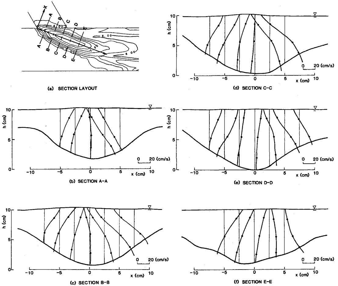
Fig.4 Secondary flow in the scour hole
