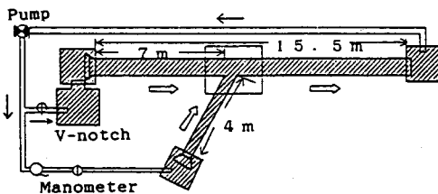
Fig. 1 Experimental apparatus
