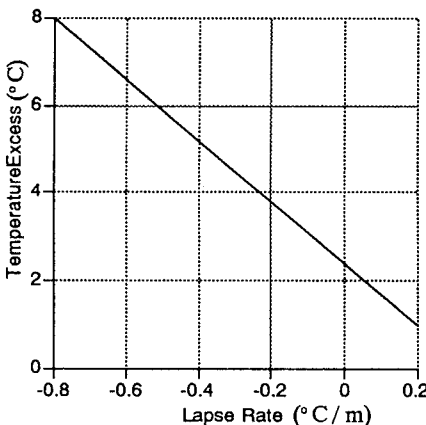
Figure 4: Relation between heat island intensity and vertical temperature gradient, adapted from Ludwig.
