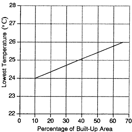
Figure 3: Relation between lowest temperature and percent of built-up area for summer days in Nagoya, adapted from Mizutori.
