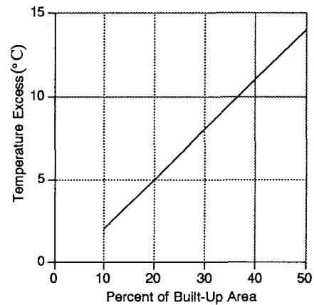
Figure 2: Relation between heat island intensity and percent of built-up area in Maryland
