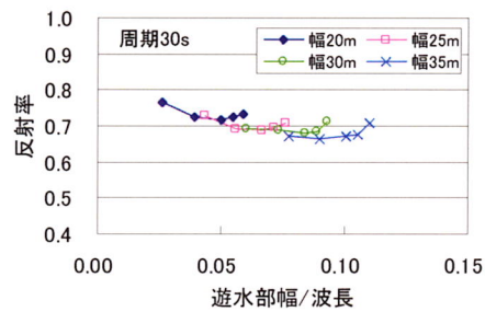
(a) 周期30s
