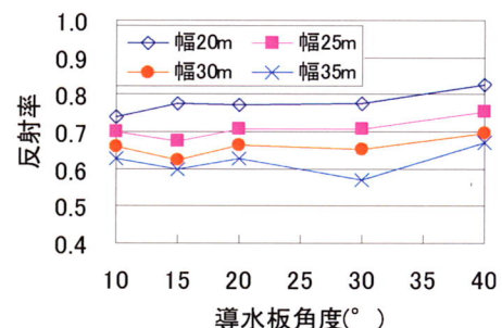
図-10 導水板角度と反射率の関係 (周期60s)
