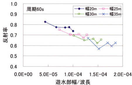
(b) 周期60s
