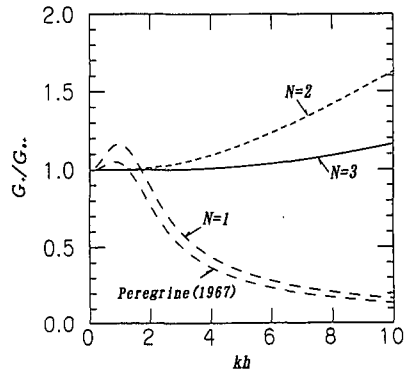
図-4 2次非線形干渉特性 (superharmonics)
