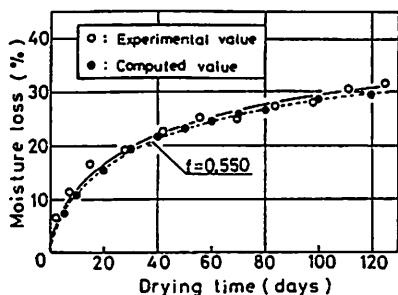
FIG. 9 Determination of surface factor
