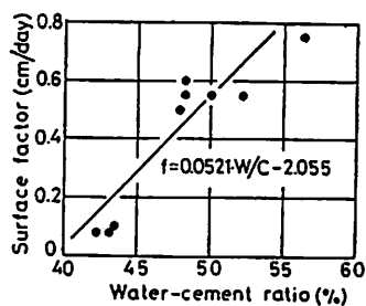
FIG. 10 The relationship between surface factor and water-cement ratio of concrete
