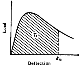
Fig. 3 Flexural toughness.
