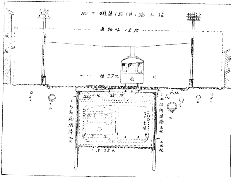
(3) Cross Section of Underground Railway, under Construction
