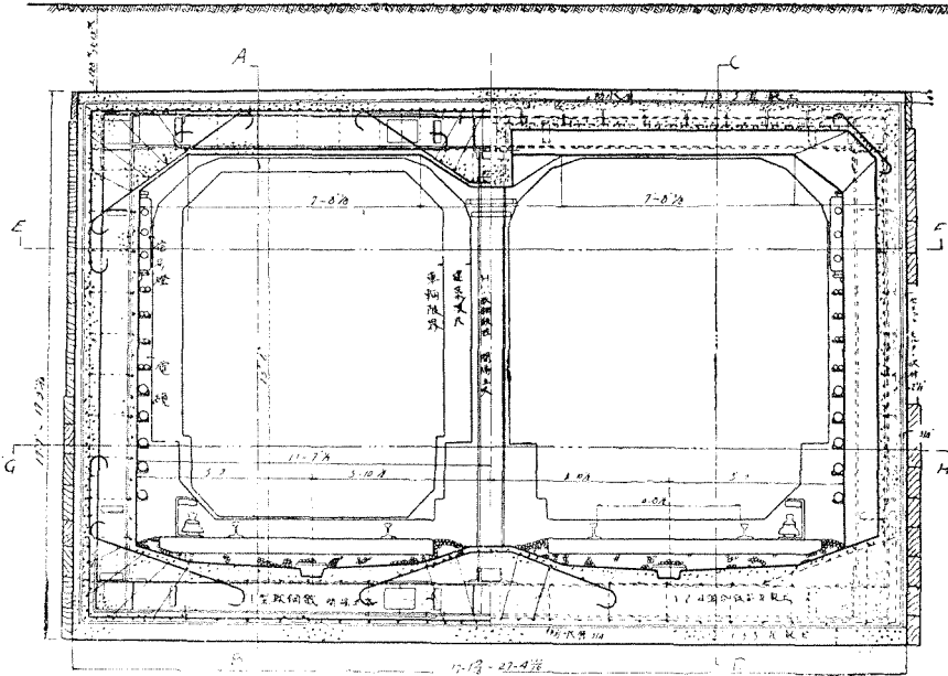
(24) Cross Section of Tunnel
