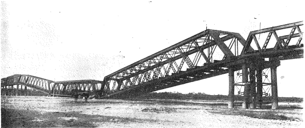
(1) Damage on piers of the Nagaragawa-Railway bridge.
