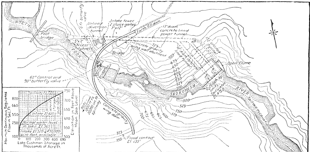
(2) Plan of lake Cushman Dam, Power house, Intake, and Tunnels.
