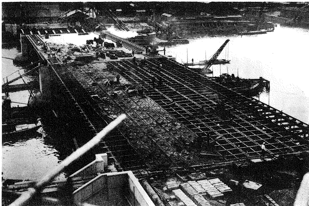
The Kurumaye Bridge Under Flooring Work.
