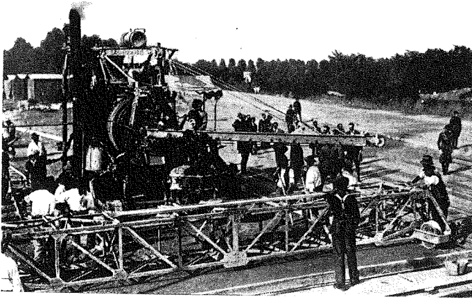
(1) A Concrete Mixing Machine at Work.
