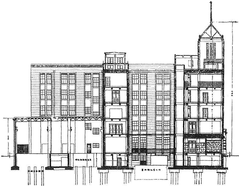
Cross Section of the Building.
