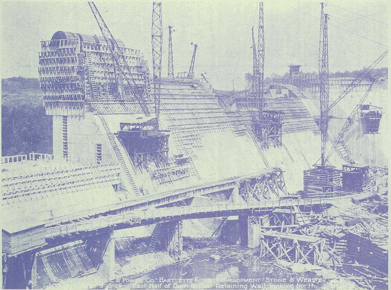
Columbus Electric & Power Co.-Bartlett's Ferry Development-Stone & Webster, Inc., Builders. East Half of Dam & East Retaining Wall, looking North. September 15th, 1925.
