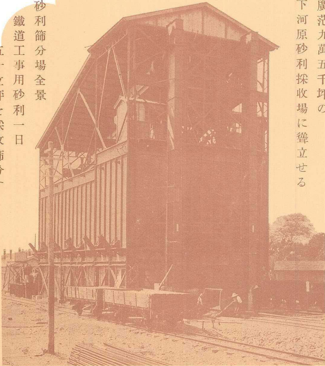
THE STORAGE AND SCREENING PLANT OF THE IMPERIAL GOVERNMENT RAILWAYS AT SHIMOGAWARA ON THE TAMA RIVER NEAR TOKYO. THE CAPACITY OF THE PLANT IS 500 TONS PER DAY.
