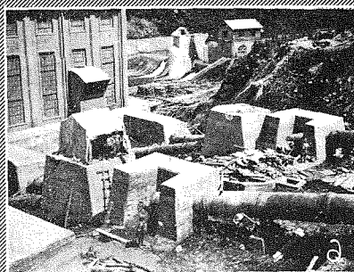
(7) Bursting Pit. Order of Setting the Bursting Pit. #1 Assembling of Bursting Pit. #2 Excavation for the Foundation. #3 Setting. #4 Setting. #5 Setting. #6 Setting Completed and Concreted.
