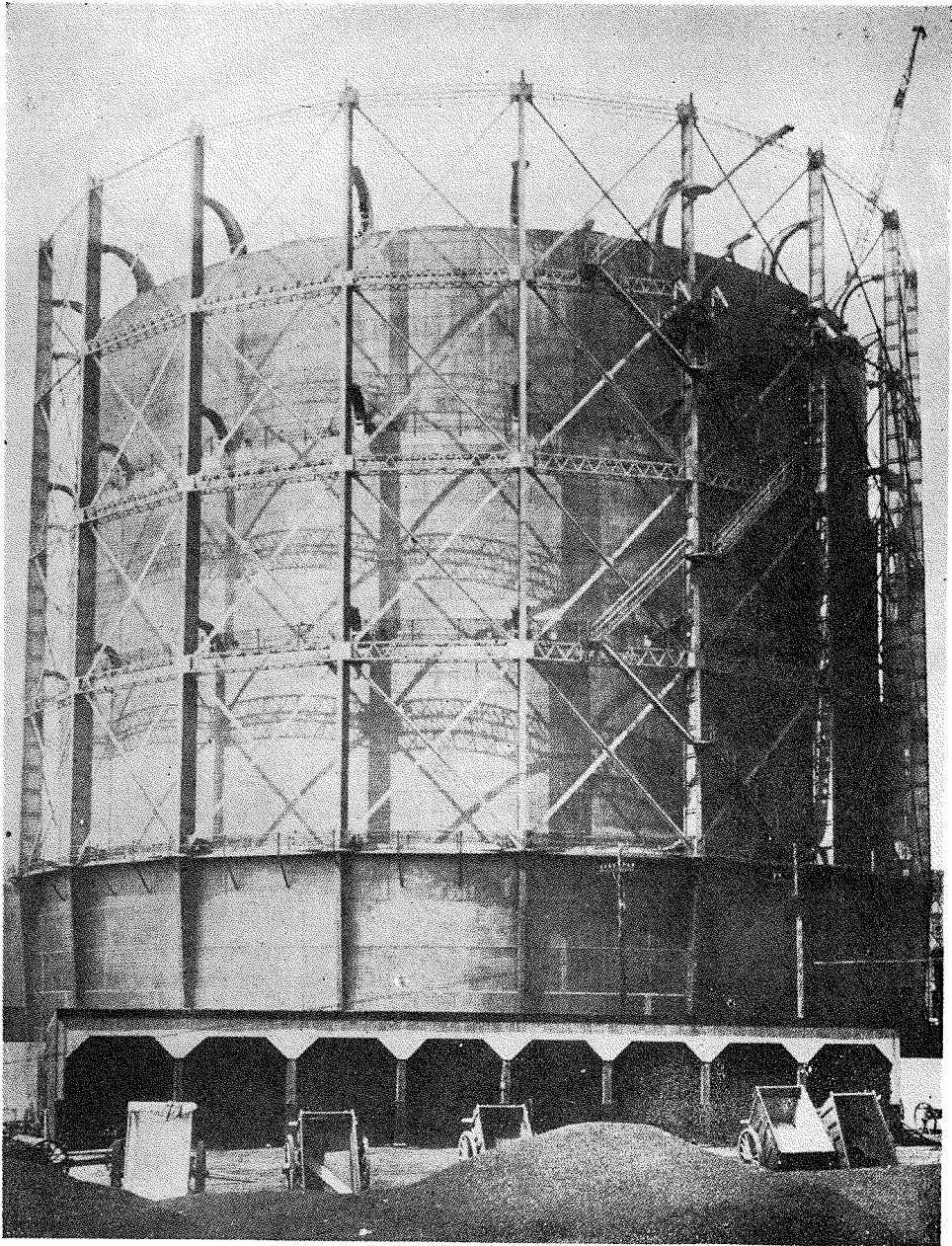
Gas Holder 〓 New Haven Gas Light Company.
