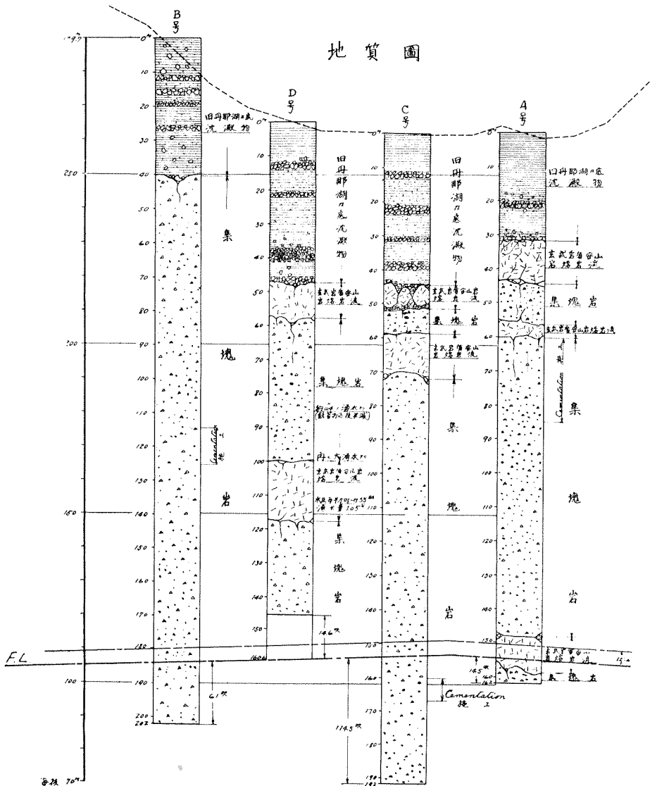
Sketch of Four Borings made at the Tanna Tunnel Site.
