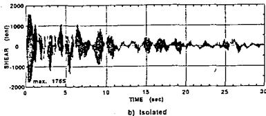
Fig. 4 Base Shear Response
