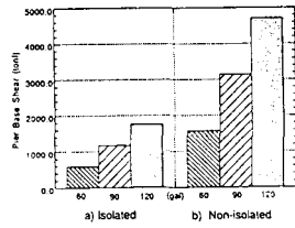
Fig. 7 Max. Pier Base Shear and Moment
