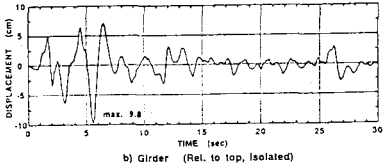
b) Girder (Rel. to top, Isolated)
