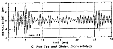
Fig. 2 Displacement Response
