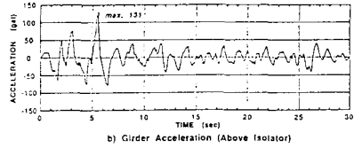
b) Girder Acceleration (Above Isolator)
