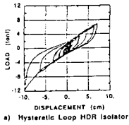
a) Hysteretic Loop HDR Isolator
