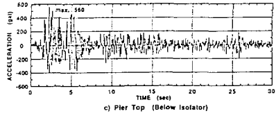
Fig. 3 Acceleration Response
