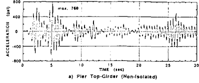
a) Pier Top-Girder (Non-Isolated)
