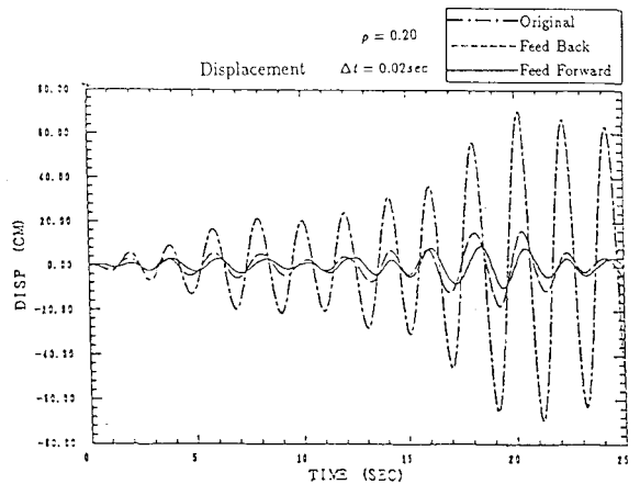
Fig.4 Simulated Response
