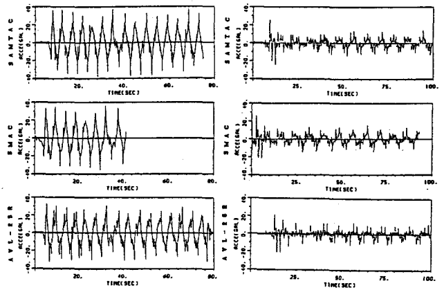
(a) G015 (b) I005 Fig. 2 Corrected Accelegrams
