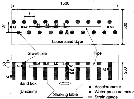
Fig.11 General view of test apparatus.
