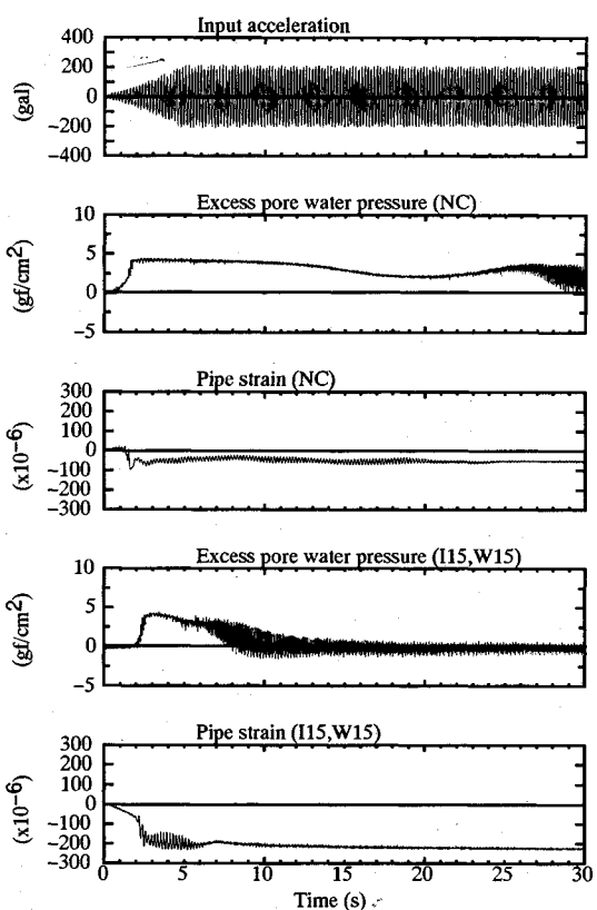
Fig.17 Time histories of input acceleration, excess pore water pressure and pipe strain (1 gal = 10 -2 m/s 2 , 1 gf/cm 2 = 98 Pa).
