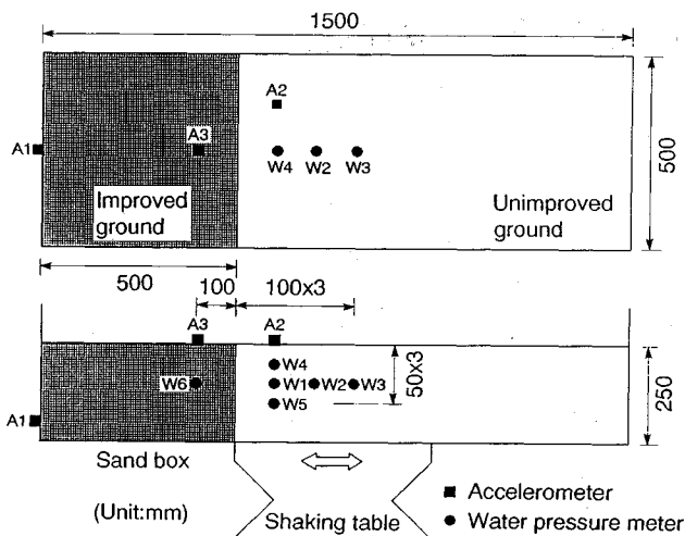
Fig.1 General view of test apparatus.
