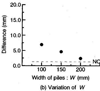
Fig.14 Difference of settlement between inner and outer ground surrounded by gravel piles.
