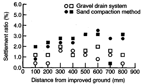
Fig.7 Settlement ratio in relation to distance from improved ground for 80 gal (0.8 m/s 2 ) input acceleration.
