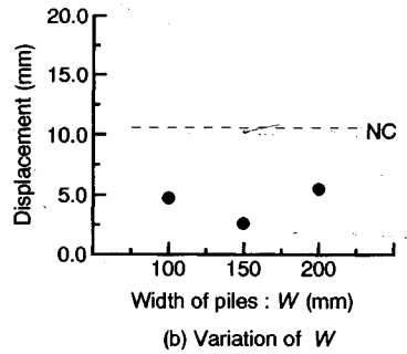
Fig.15 Vertical displacement of pipe.
