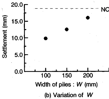
Fig.13 Settlement of inner ground surrounded by gravel piles.
