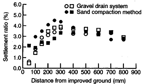
Fig.8 Settlement ratio in relation to distance from improved ground for 100 gal (1.0 m/s 2 ) input acceleration.
