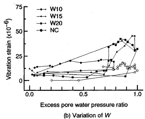
Fig.18 Relationship between excess pore water pressure ratio and vibration strain.
