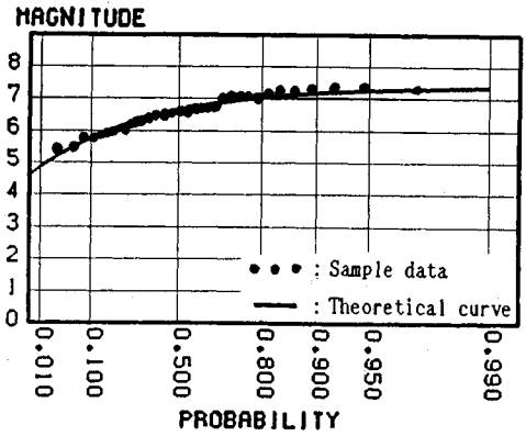
Fig.11 Distribution of 50-year maximum of magnitude (Cluster 2, Energy level=Middle)
