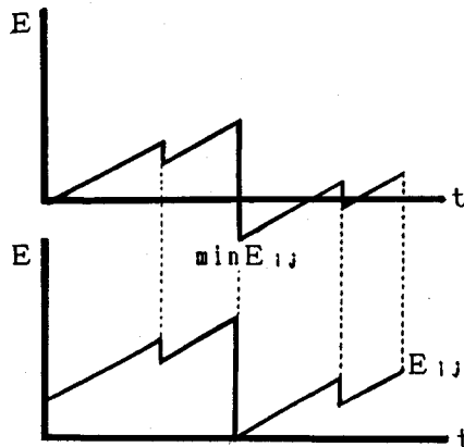
Fig.4 Parallel movement of the strain energy-time curve
