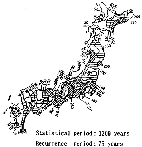
Fig.16 Seismic risk map by Gotou and Kameda
