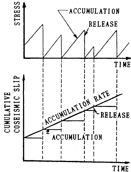
Fig.2 Slip-predictable model
