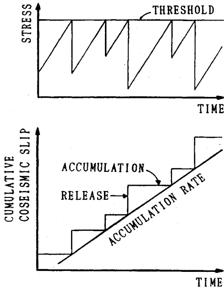
Fig.1 Time-predictable model
