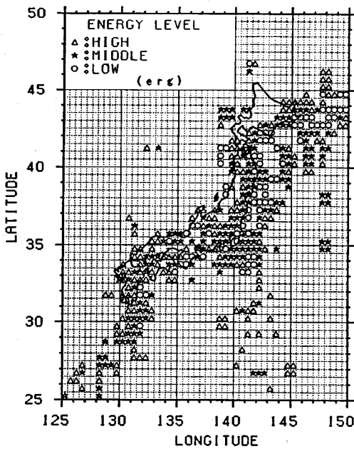
Fig.7 Strain energy accumulation (Cluster 1)
