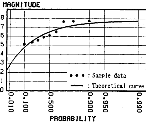
Fig.10 Distribution of 50-year maximum of magnitude (Cluster 3)
