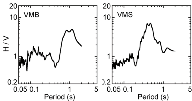
Figure10. H/V of microtremors measurements near strong motion station Viña del mar Centro [VMS], and within the building damage area [VMB] in Viña del mar
