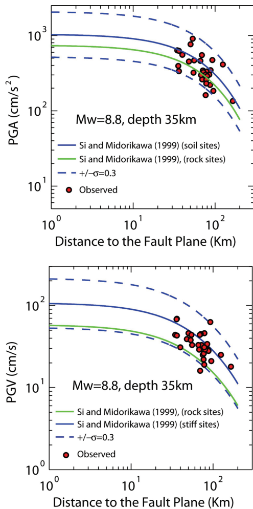
Figure 5. Attenuation of PGA and PGV for observed strong motions Maule mega-earthquake (Chile)
