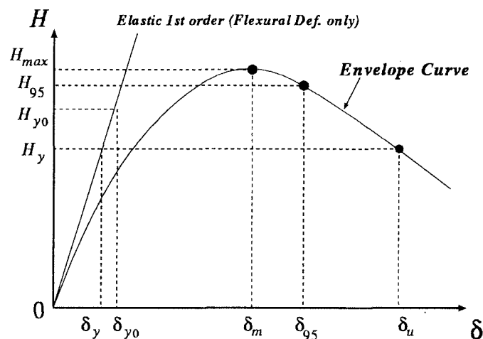
図-3.1 Definition of Loads and Displacements
