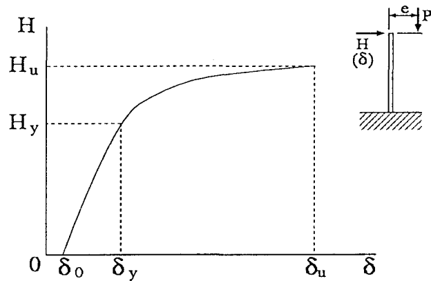
(b) Eccentrically loaded vertical force
