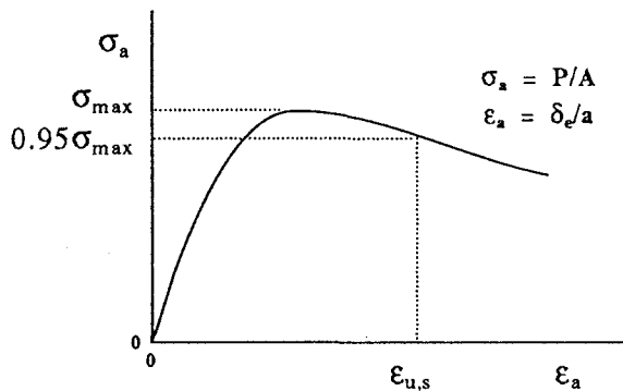
(b) Average stress-average strain relation
